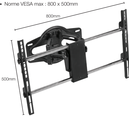
Ref. 903086 Bras pivotant mural 37-50"
