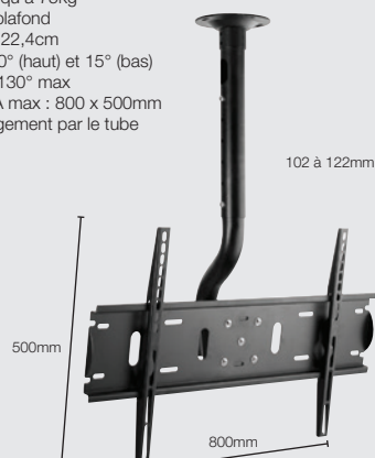
Ref. 903231 Support plafond 37-60"
