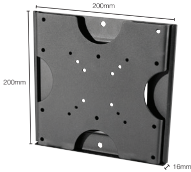
Ref. 903033 Support mural 15-32"
